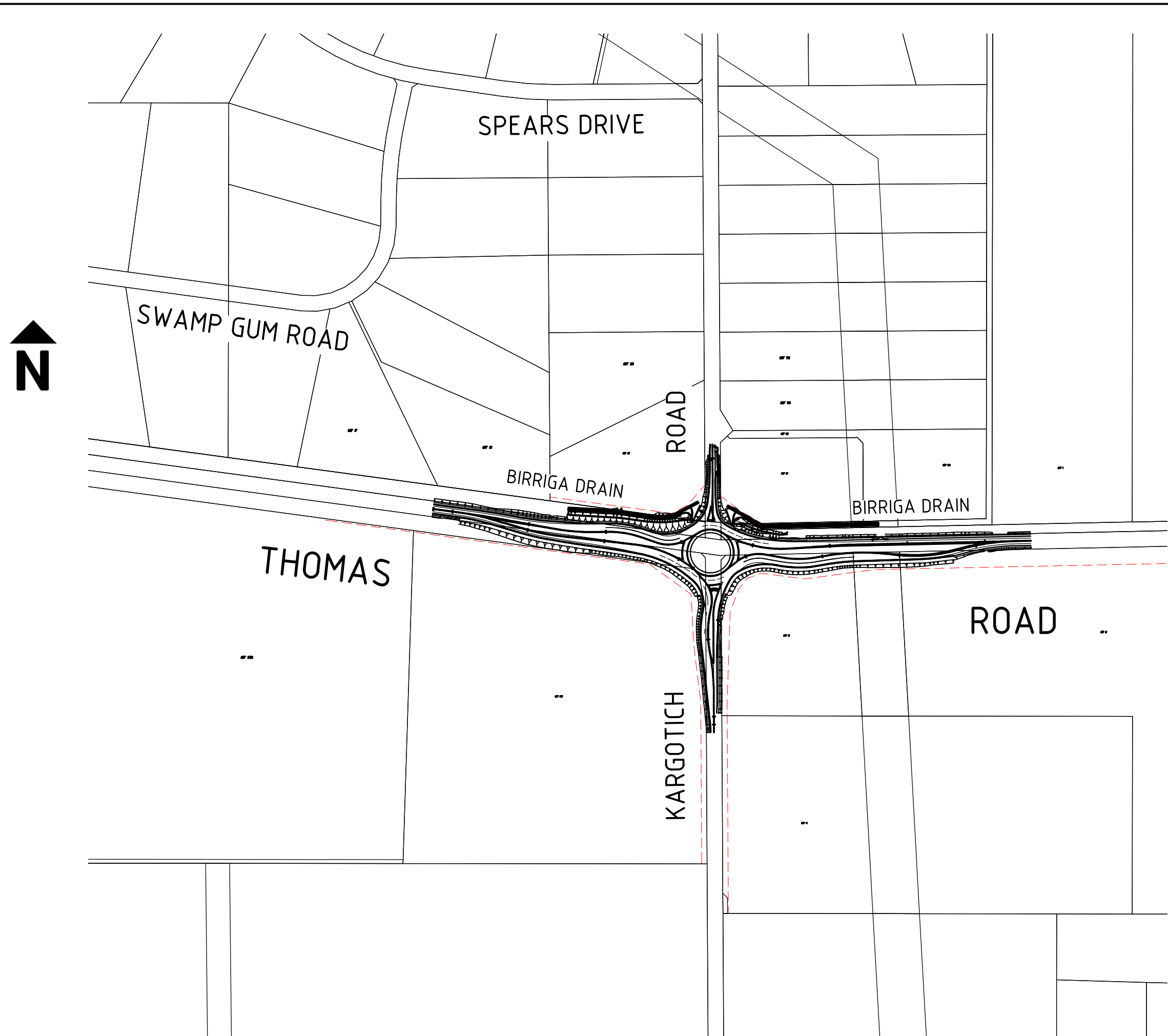
KEY PLAN 1:5000
