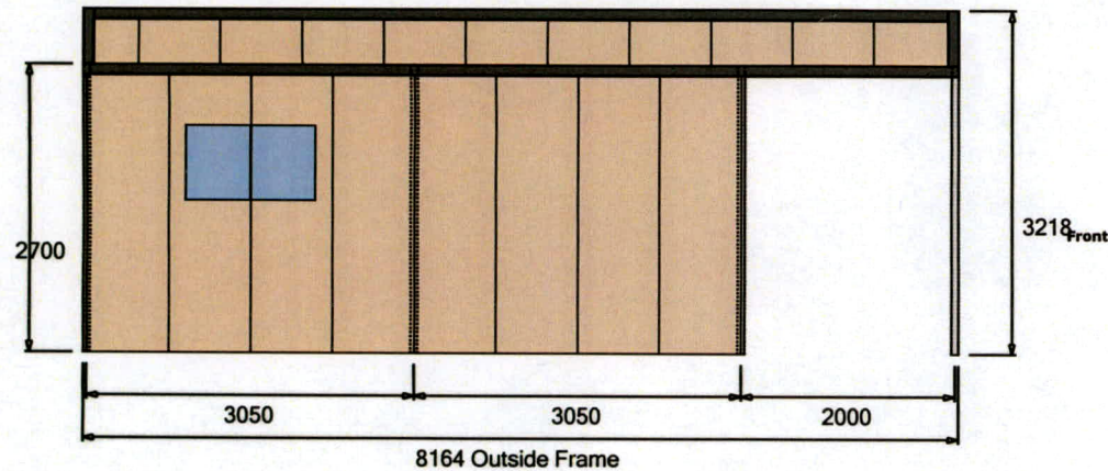
Left Elevation
