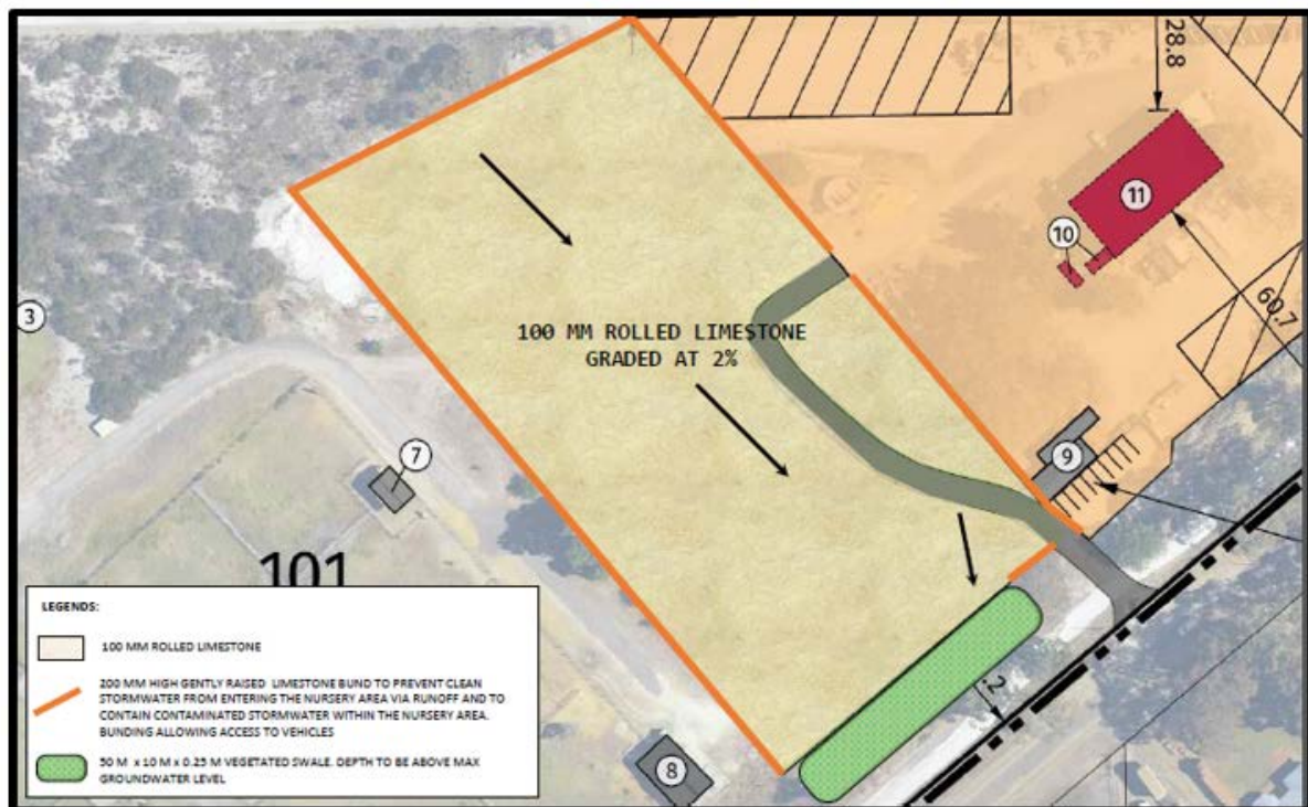
Figure 3: Run off and Stormwater Management
