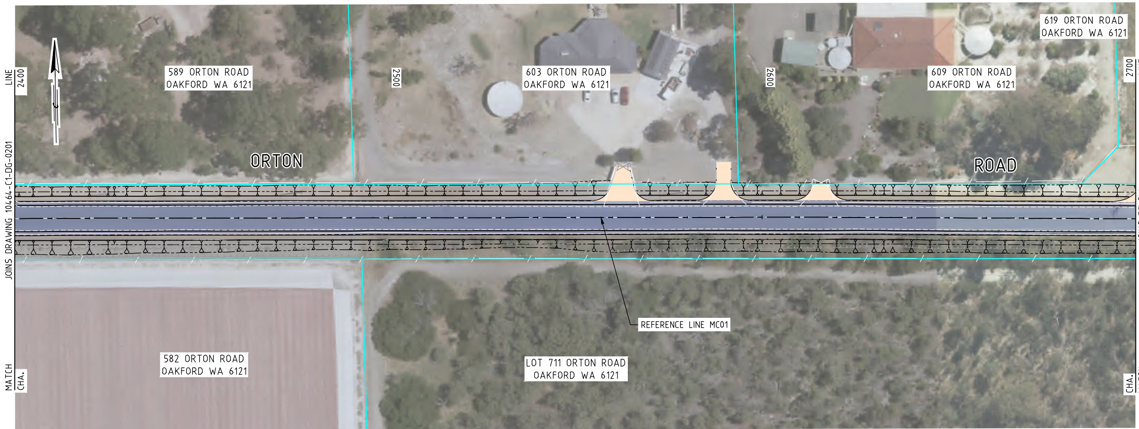
PLAN (MC01) 1:500
